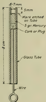
FIG. 173.—Method of Filling K. & S. Fusing-Point Tubes.
